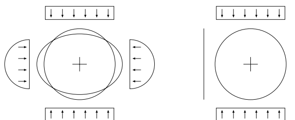
Figura 9-1 Tubo flexible
